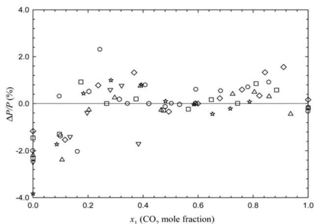
Fig. 3. Deviation of pressure for the system CO 2 (1)+HFC-143a (2) from the PR- EoS using W-S mixing rule at 273.15 K (◆); 283.15 K (□); 293.15 K (○); 303.15 K (△); 313.15 K (☆); 323.15 K (○); 333.15 K (▽).
